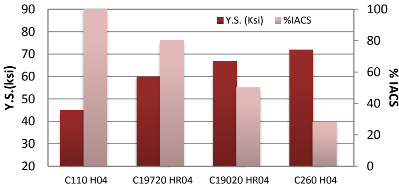
Figure 1: Comparison of Yield Strength and Electrical Conductivity performance of select automotive connector materials.
